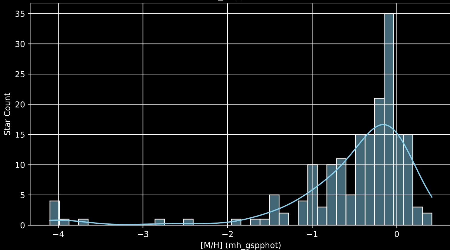
APOGEE DR17 Field: [203+04-RV_btx [M/H] (mh_gspphot) (n= 182)
