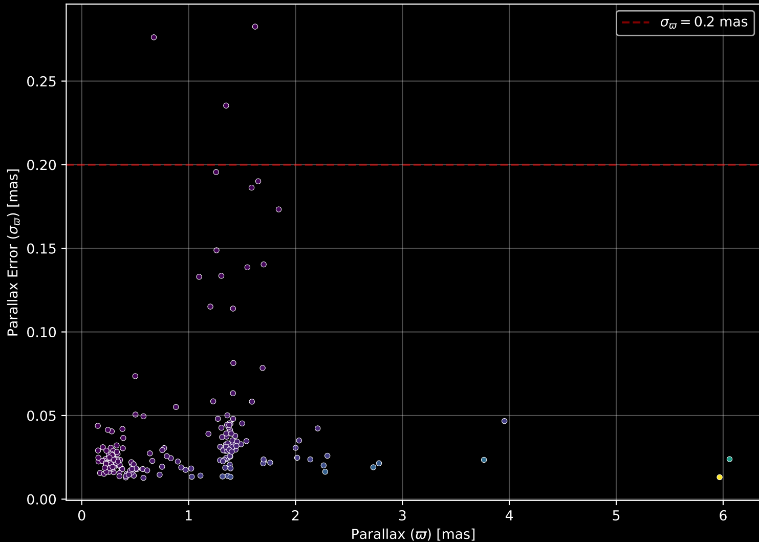
APOGEE DR17 Field: [203+04-RV_btx] Parallax Quality (n= 185)
