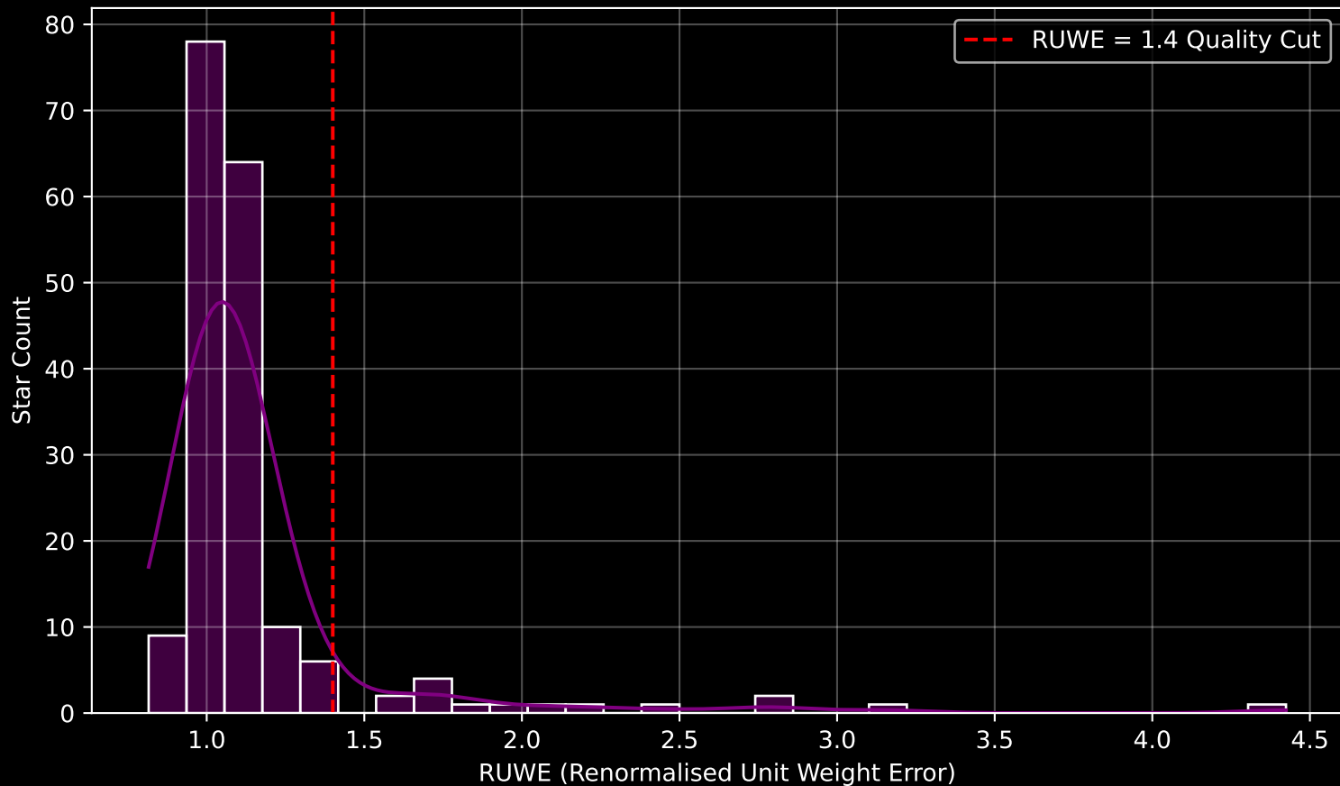
GAPOGEE DR17 Field [203+04-RV_btx] RUWE Distribution (n= 182)
