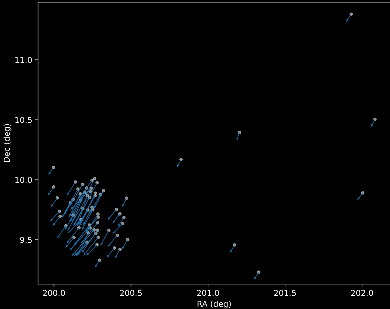
APOGEE DR17 Cluster 0 Proper Motion Vectors (n=64)
