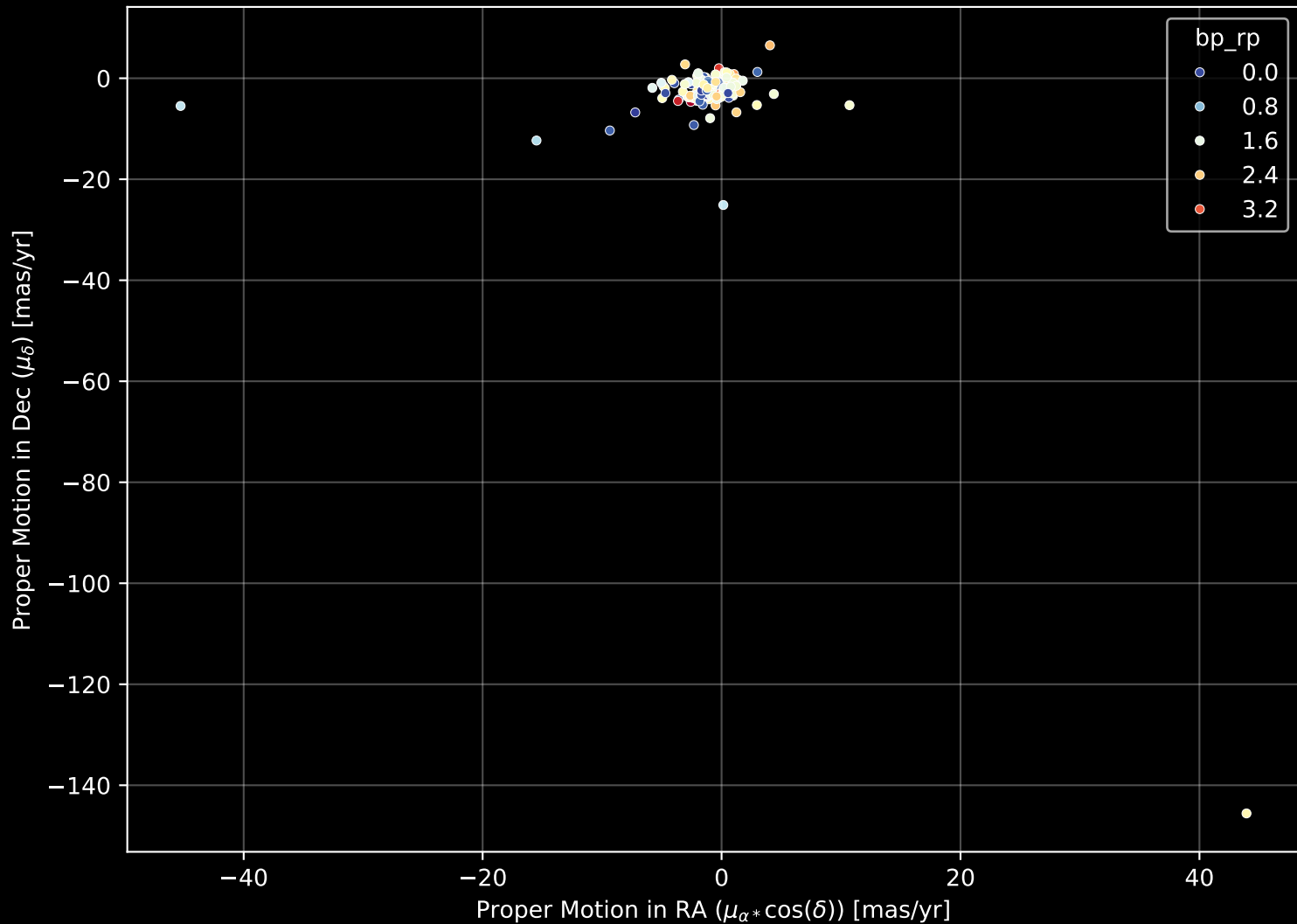
APOGEE DR17 Field: [203+04-RV_btx] Proper Motion Diagram (n= 185)
