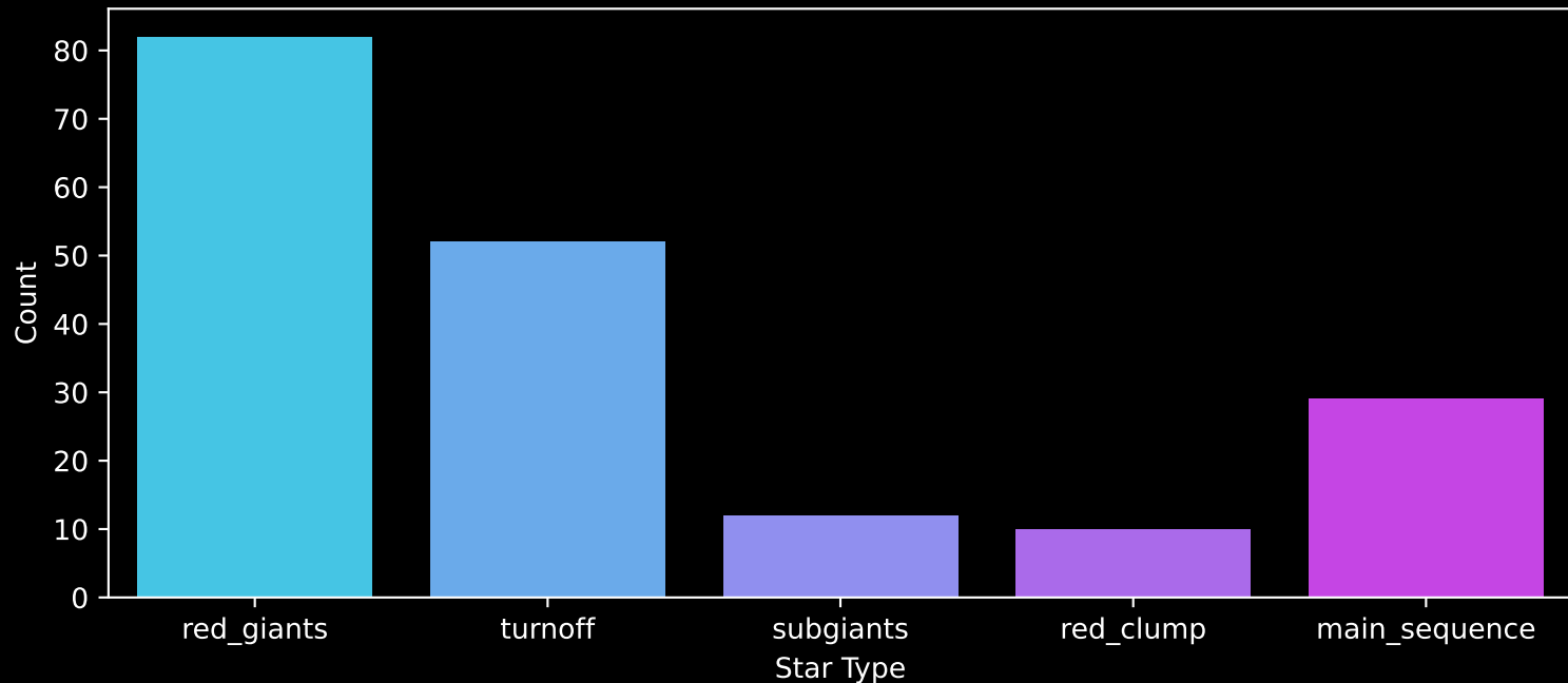
APOGEE DR17 Field: [203+04-RV_btx] Count plot of Star Type
